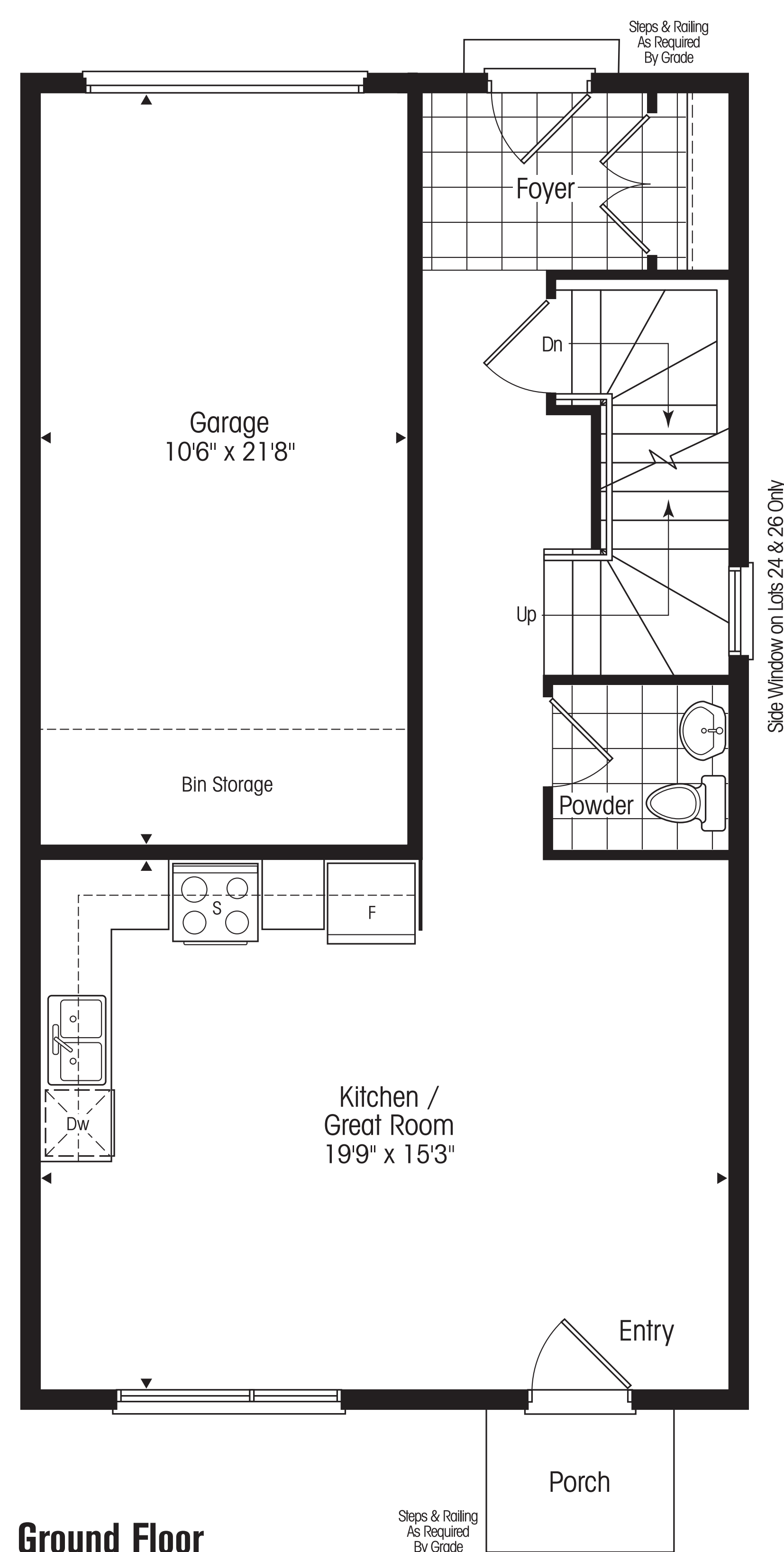
Ground Floor
