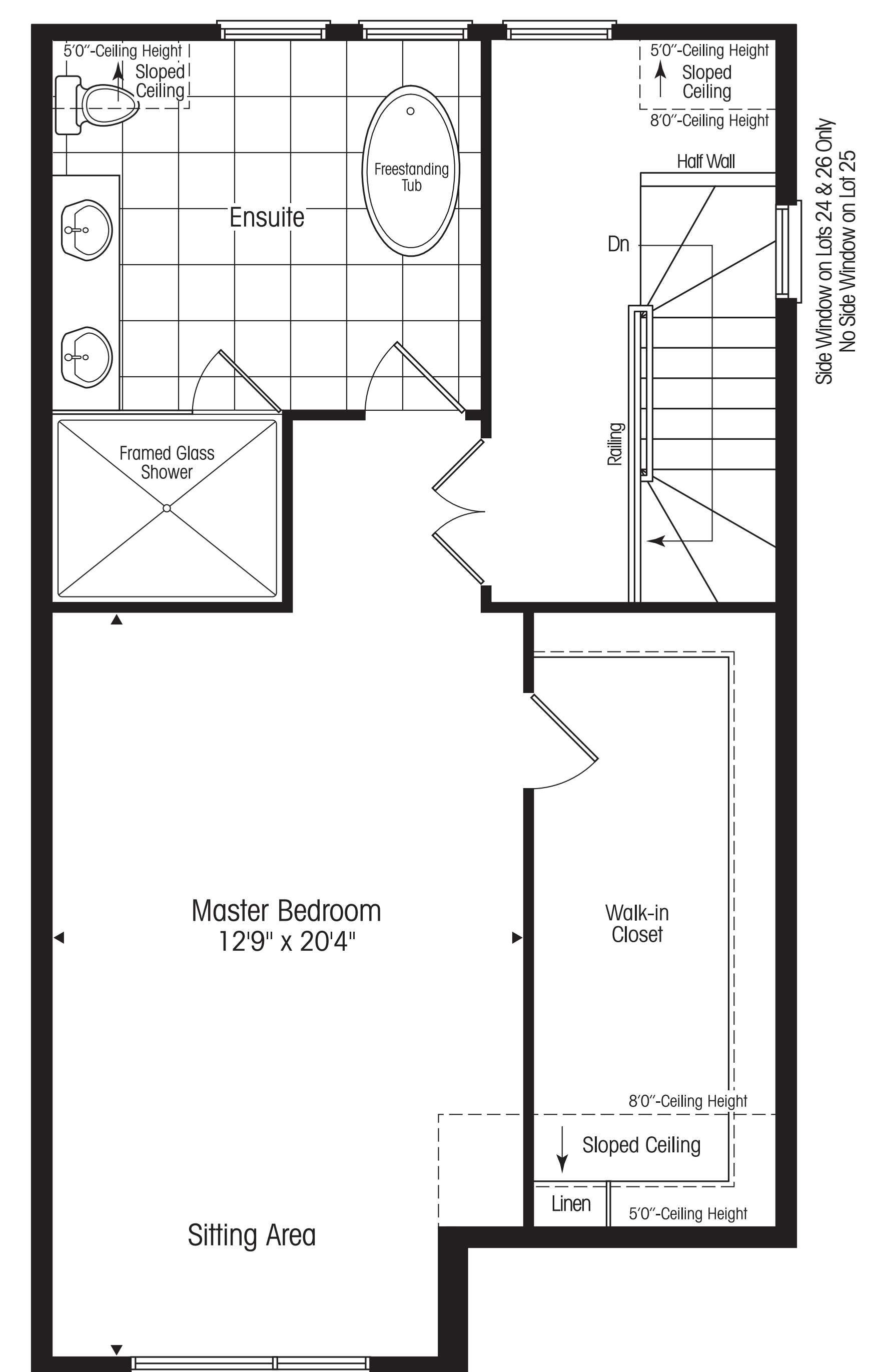
Third Floor
