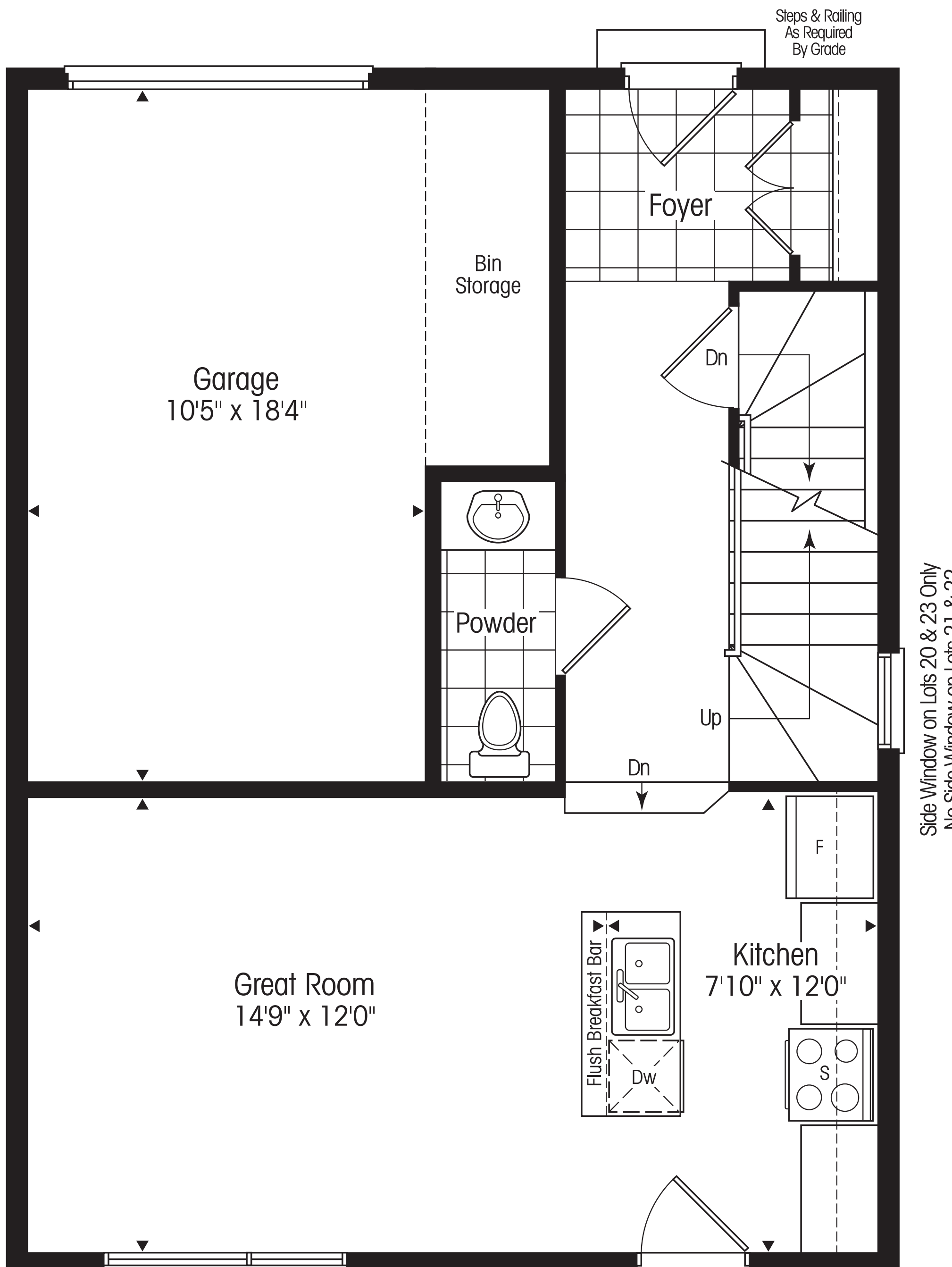
Ground Floor
