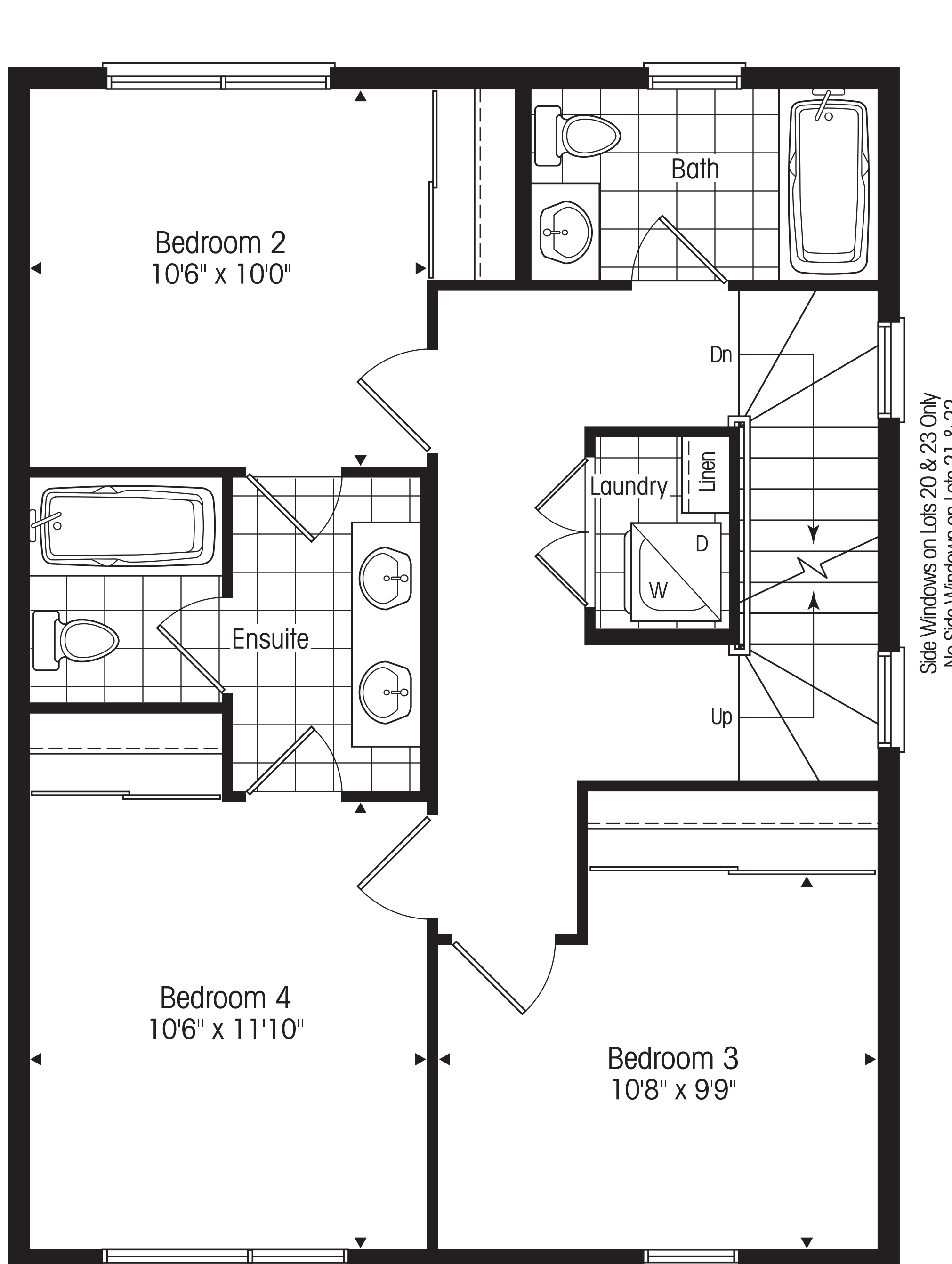
Second Floor
